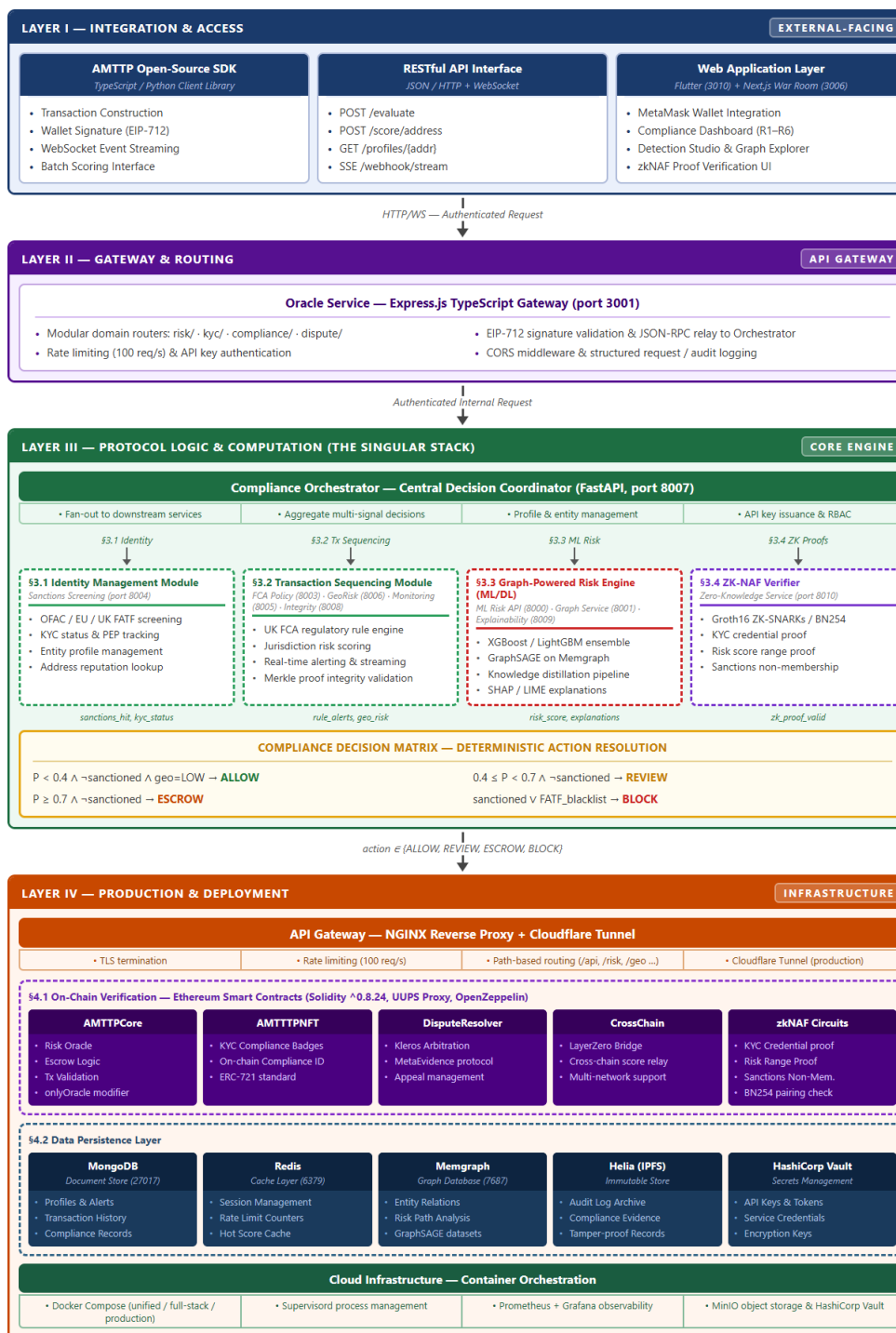
Figure 2: Four-layer architecture: Flutter/Next.js frontends, Express gateway, nine FastAPI services, Solidity contracts.
